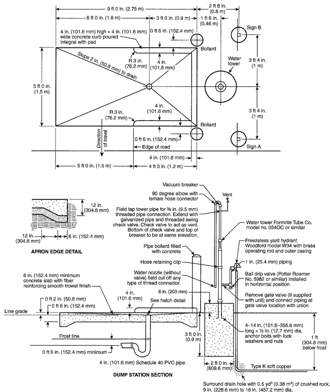
Δ FIGURE B.1(h) Optional Arrangement for a Sanitary Disposal Station on a Recreational Vehicle Park or Campground.
